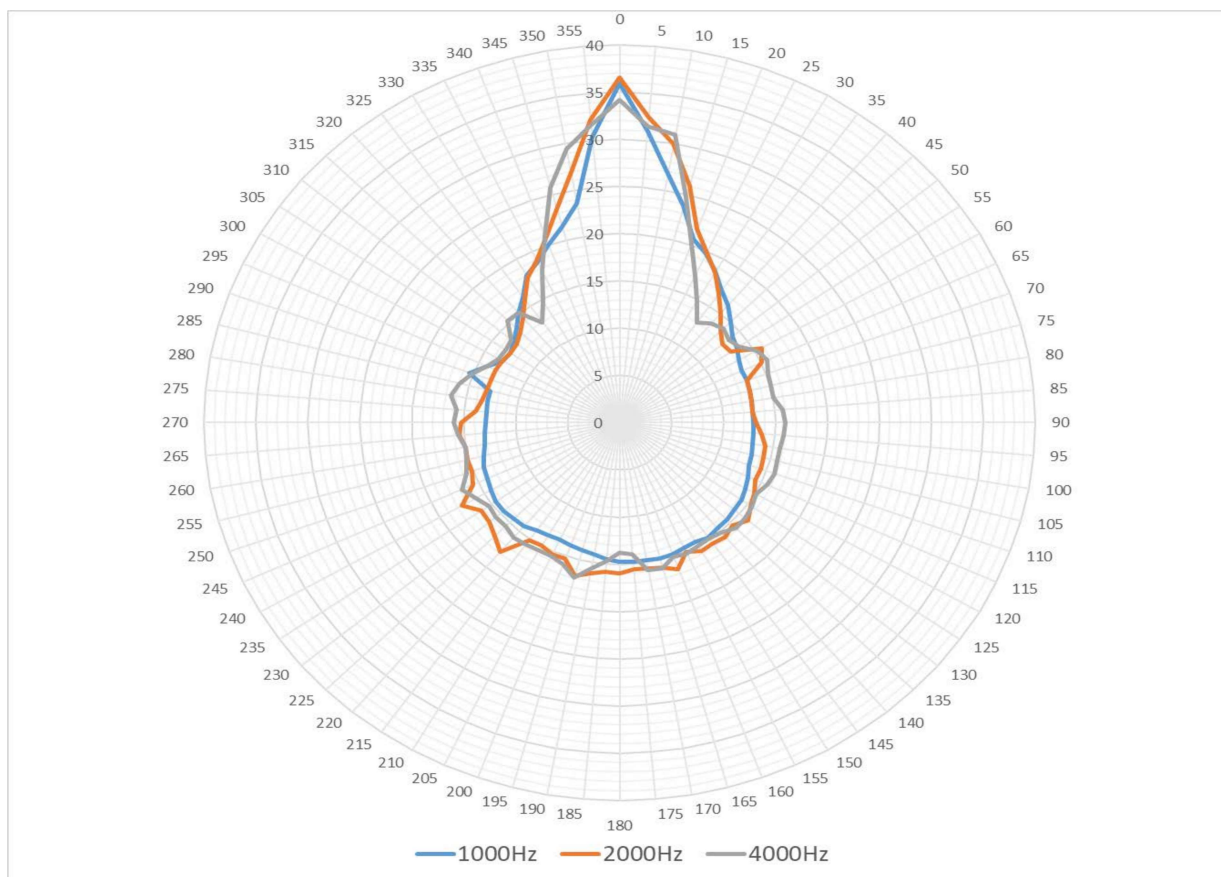
Polar Pattern
