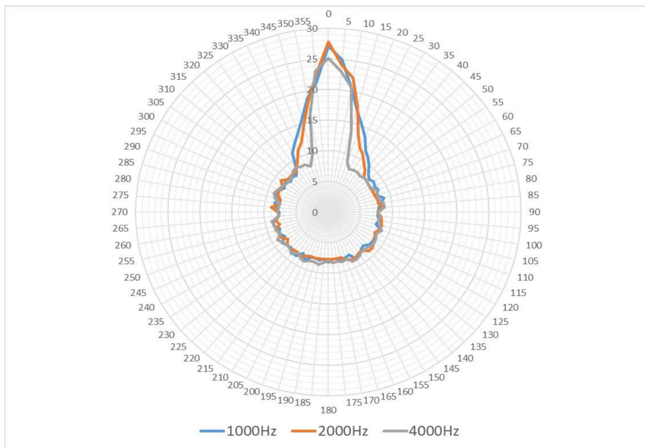
Polar Pattern
